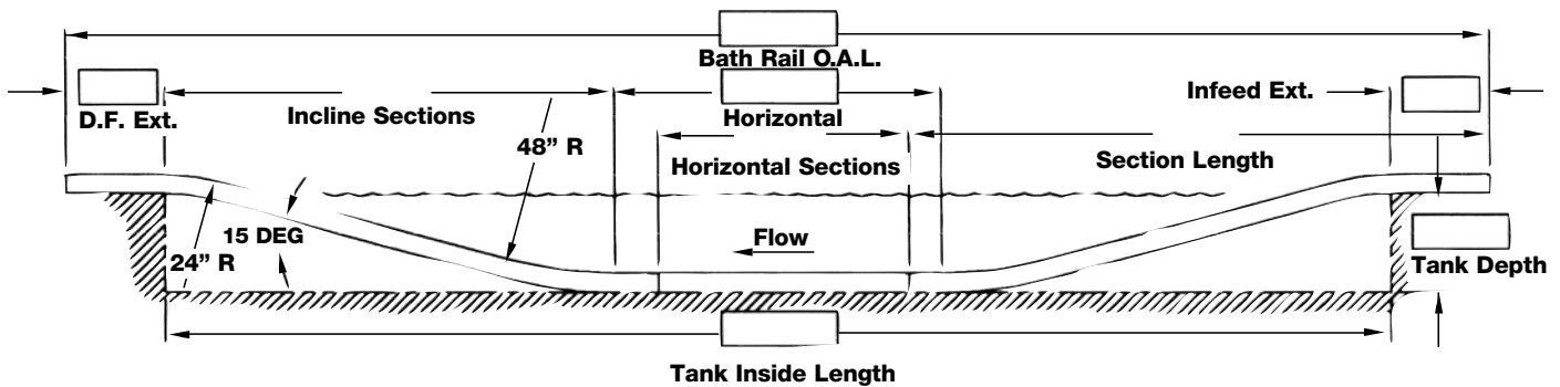
Typical Aerosol Test Bath Rail application to check for leakers and empty cans.
